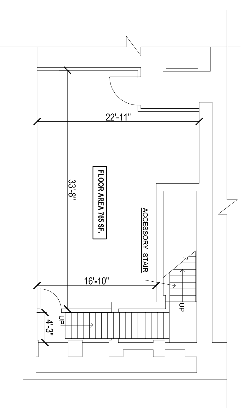
SOUTHERN RETAIL STORE LOCATED AT 579 BROADWAY - SUB-CELLAR LAYOUT SCALE: 1/8" = 1'-0"
