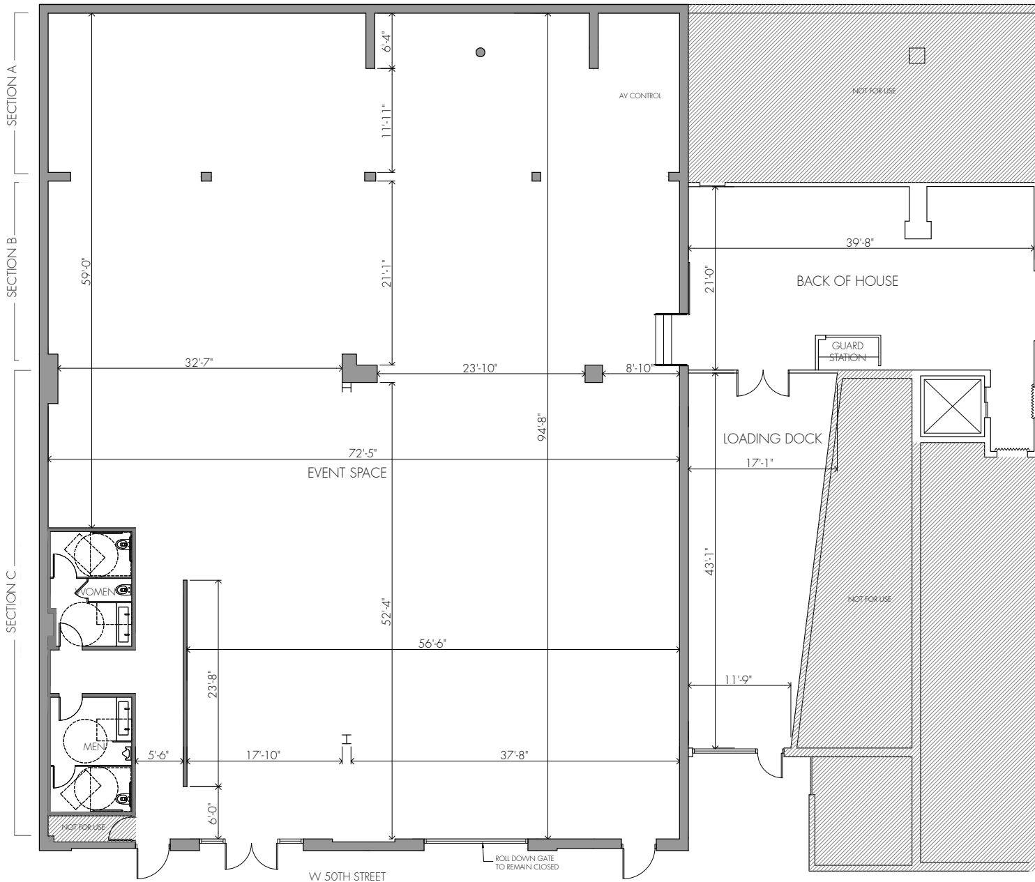
FIRST FLOOR
